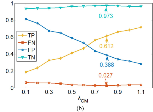
Fig. 9. Impact of different \lambda_{CM} on prediction error: (a) supervised loss and confusion matrix loss, (b) components of the confusion matrix.
